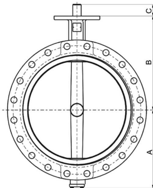
Fit DN400-DN1200 U-Type Butterfly valves
