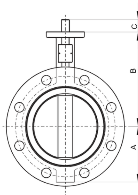
Fit DN40-DN350 U-Type Butterfly Valves
