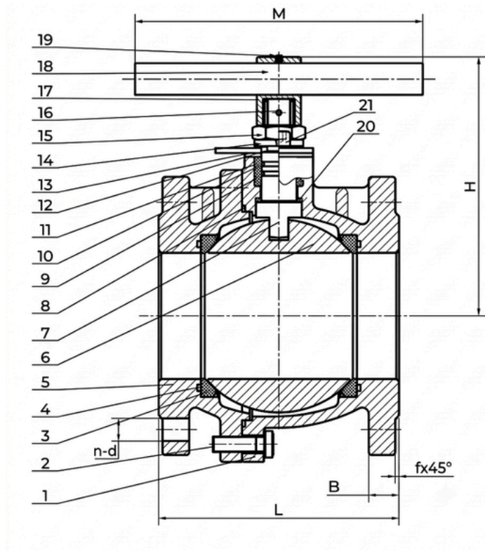
DN100-DN200
