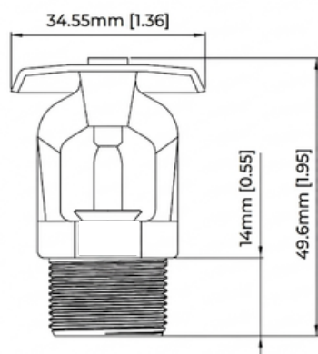
Upright Sprinkler
