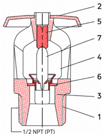
BL 5601 & BL 5603 (Standard Response)
