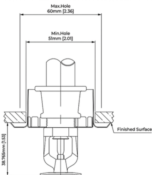
Maximum Extension
