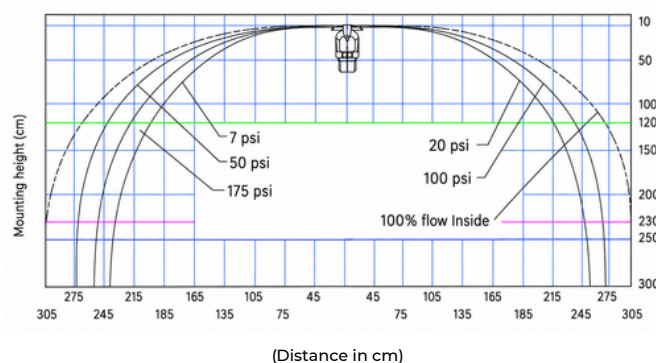
Distribution Pattern (Upright)
