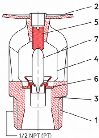
BL 5601 & BL 5603 (Standard Response)
