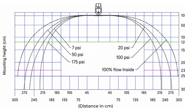
Distribution Pattern (Pendent)
