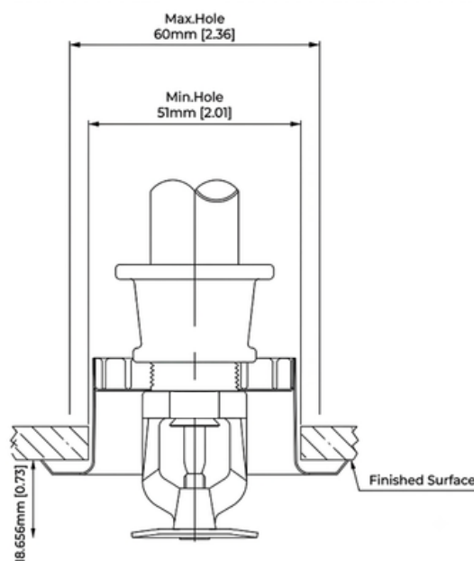
Maximum Recess
